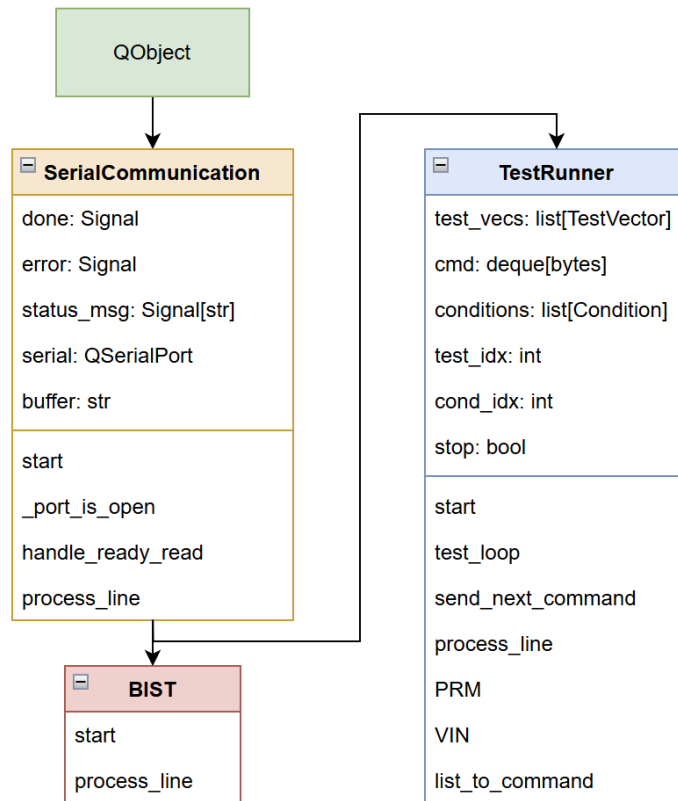
Figure 8: Basic layout of serial_communication.py
