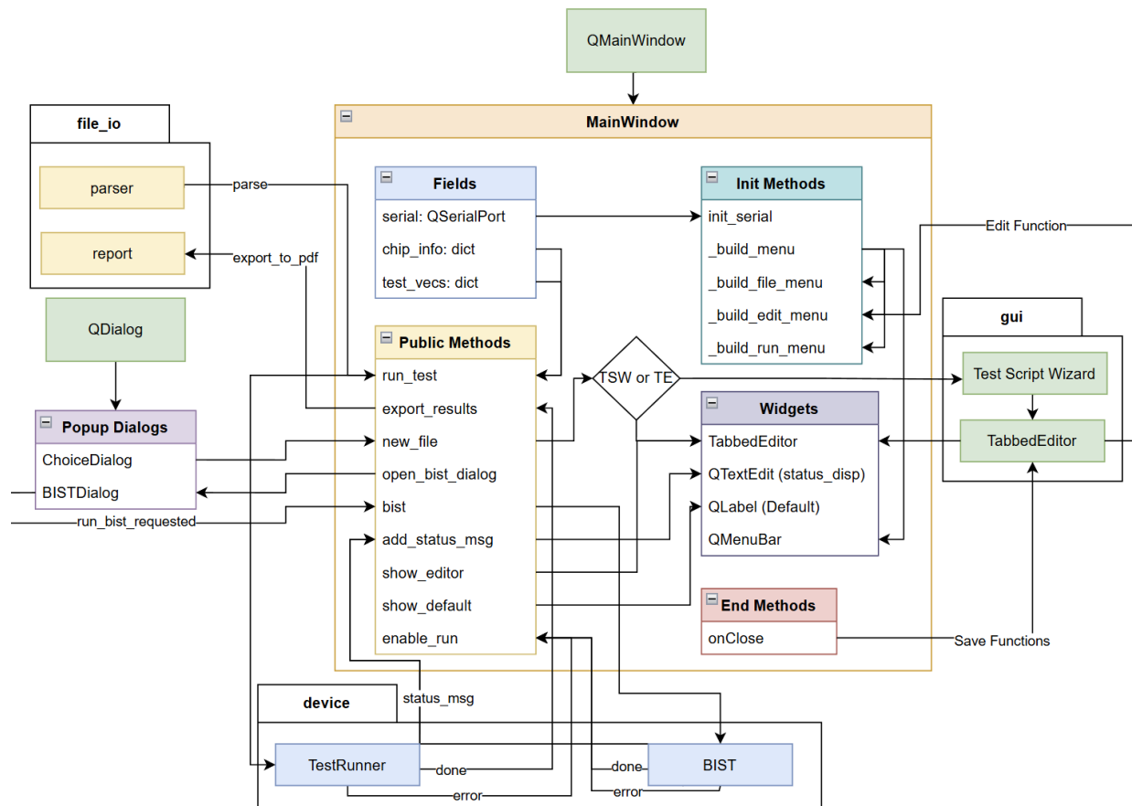
Figure 9. High level overview of the application and its connections to MainWindow
